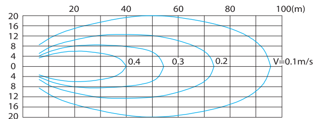
LFP5.5/4-2500-47
