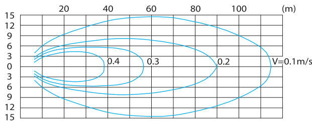
LFP7.5/4-2100-52
