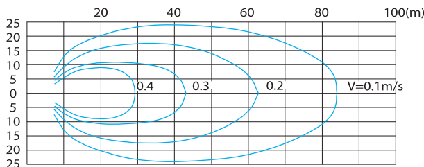
LFP4/4-2500-43
