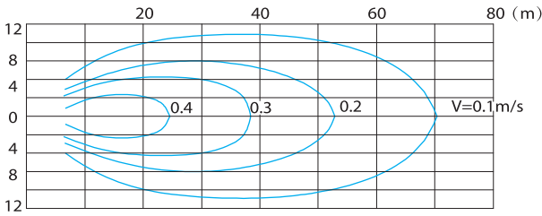
LFP4/4-2100-43
